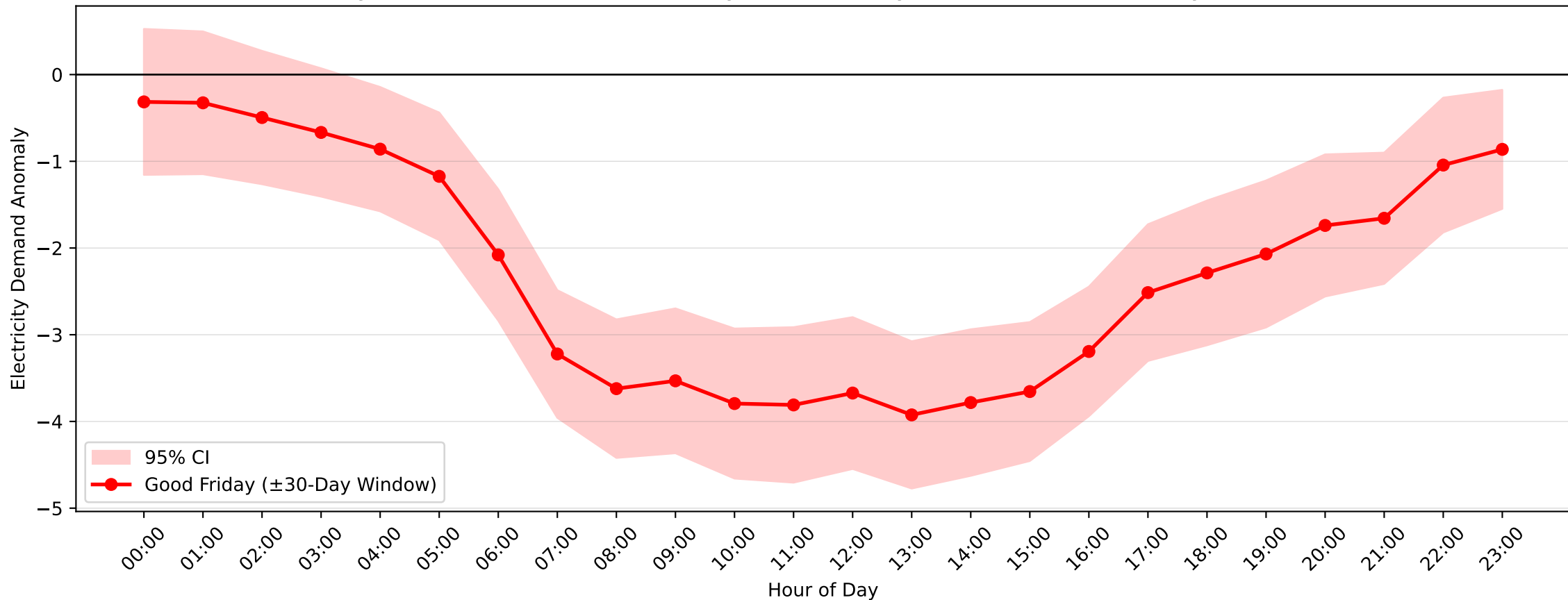
Mayfield West Demand Anomaly: Good Friday (2004–2017, \pm 30 -Day Window)
